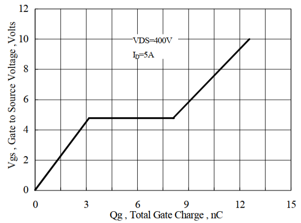
Fig 10 Gate-Charge Characteristics
